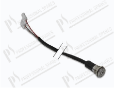
Start pushbutton with lamp Ø 19 mm cable L=740 mm; faston 6,3 mm
